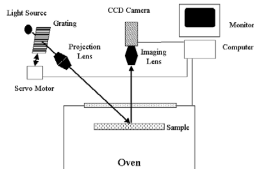
Micro Fringe Projection Configuration
